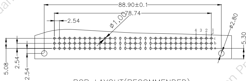
PCB LAYOUT(RECOMMENDED) (TOP VIEW TOL. :±0.05)
