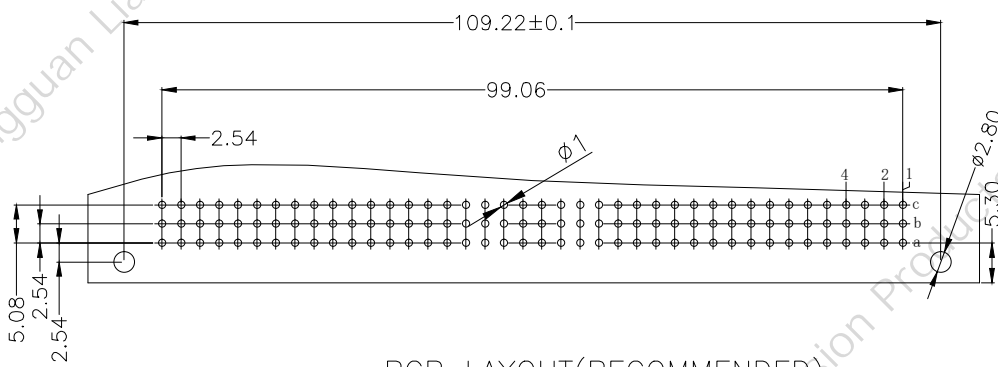
PCB LAYOUT(RECOMMENDED)
