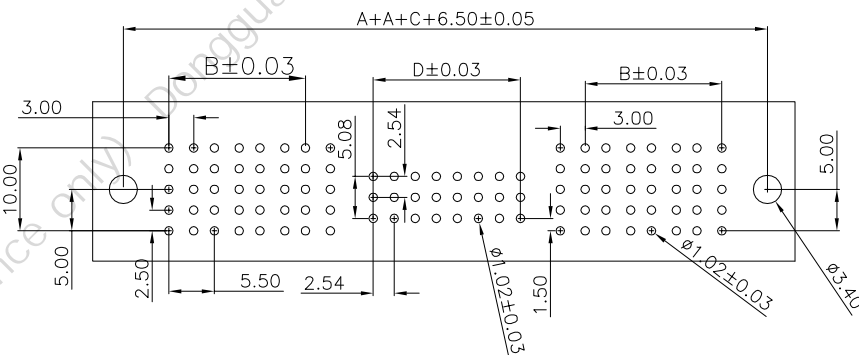
Recommended PC board pattern (TOP VIEW)
