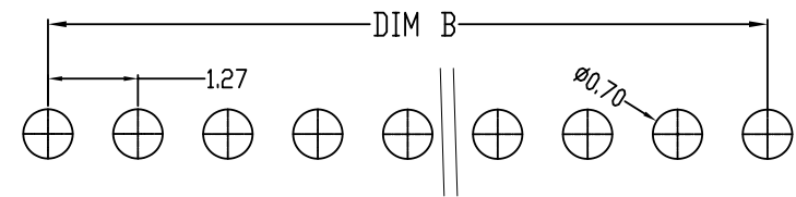
PCB LAYOUT
